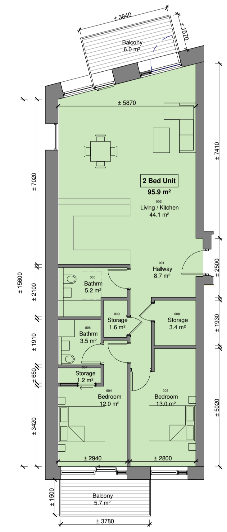
5 Unit Type - 2BR-B2 scale 1 : 100
