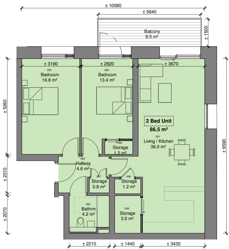
2 Unit Type - 2BR-A1 scale 1 : 100
