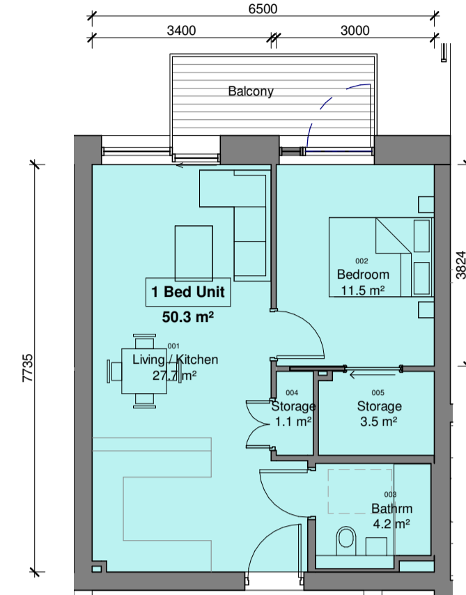
4 Part V - Unit Type - 1BR-B1 scale 1 : 100
